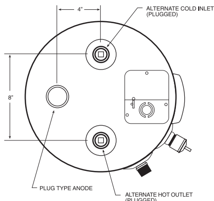
Top View 6 & 12 Gallon Models
